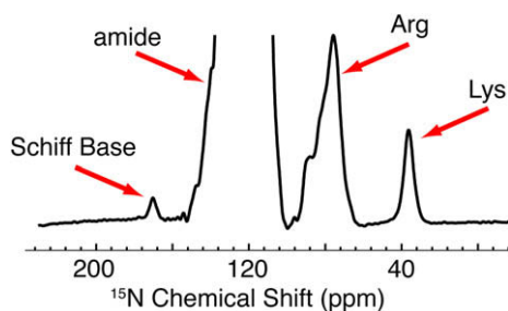
Fig. 3. 1D DNP enhanced ^{15}\text{N} spectra of bR illustrating the excellent S/N available with DNP that permits observation of the ^{15}\text{N} signal of the single Schiff Base (K216). The Arg resonances irradiated with the selective pulse are labeled and lie at \sim 80 ppm.
