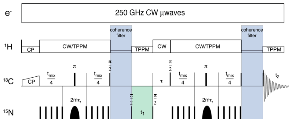
Fig. 1. Pulse sequence for ^{15}\text{N} -frequency-selective TEDOR transfer. Only ^{15}\text{N} spins within the bandwidth of the selective pulses contribute to the spin dynamics under REDOR. The sequence is described in the text. The REDOR pulses are phase cycled according to the XY-8 scheme and the overall phase cycle is documented elsewhere [1]. CW microwave irradiation was employed in the version of the experiment used to acquire the DNP enhanced spectrum.
