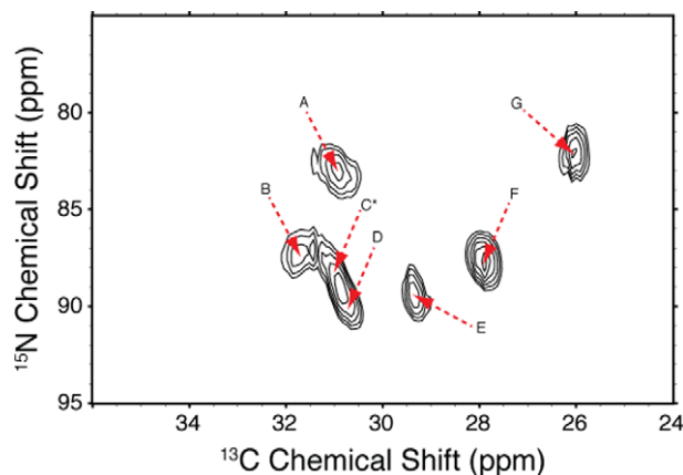
Fig. 4. 2D ^{15}\text{N} - ^{13}\text{C} selective correlation experiment focused on the Arg- ^{13}\text{C}_\gamma - ^{15}\text{N}_\epsilon of bR. The sequence described in Fig. 1 was employed with a 1.98 ms Gaussian refocusing pulse, and TPPM decoupling optimized to reduce transverse dephasing. The REDOR mixing time of 4 ms was chosen to favor short distances ( \sim 2.4 – 2.5 Å). The spinning frequency was 7.576 kHz, and all DNP experiments were conducted in dark-adapted bacteriorhodopsin (90 K), as described elsewhere.
