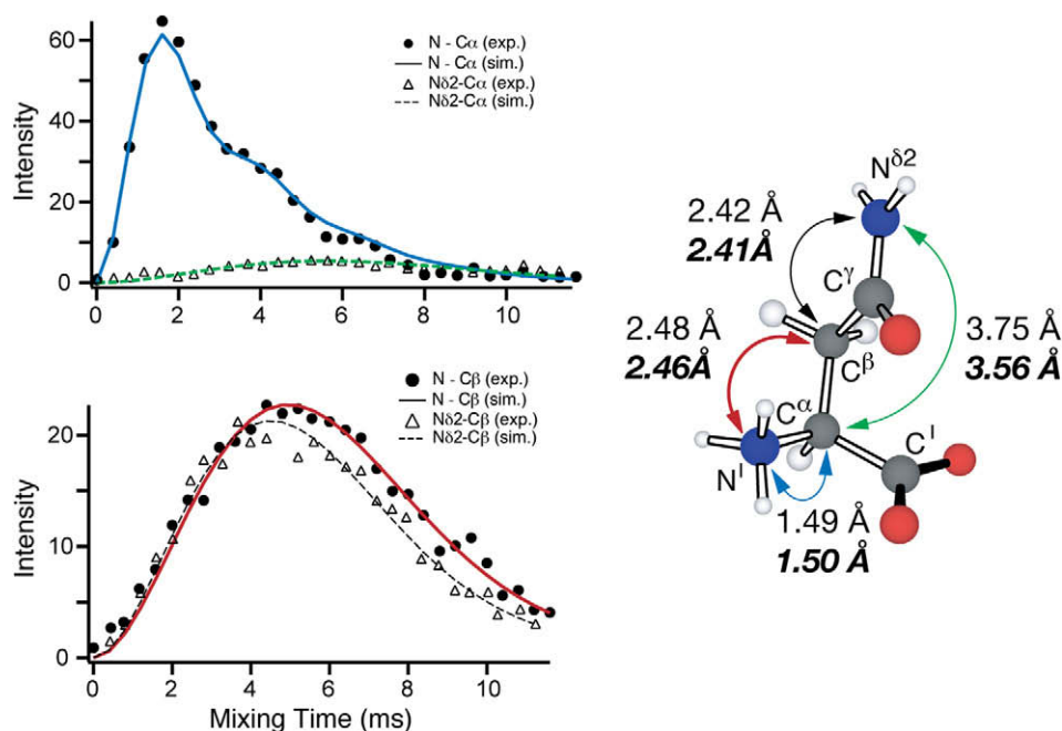
Fig. 2. FS-TEDOR experiment in 10% U-[ ^{13}\text{C} , ^{15}\text{N} ]-Asparagine. We employed 100 kHz TPPM decoupling during REDOR and other periods, a 1 ms Gaussian refocusing pulse (switched between the \text{NH}_3 and \text{NH}_2 sites), 50 kHz REDOR pulses. \omega_r 2\pi = 10 kHz.
